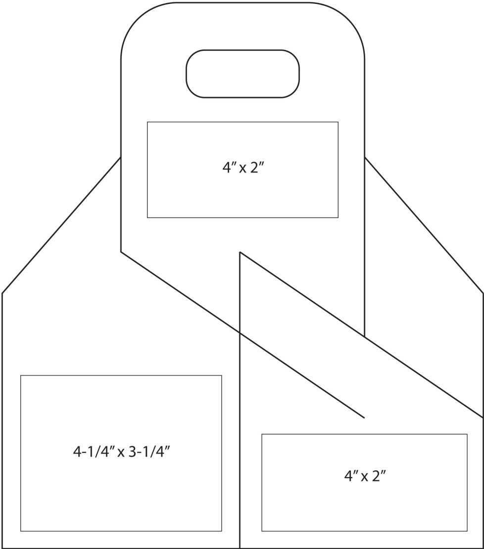
Custom Printed 4 Pack Bottle Carrier Template Dimensions: 5-1/8" x 5-1/8" x 11-3/8" to top of handle
